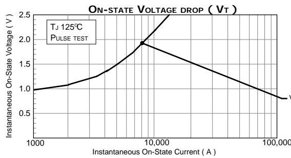
These graphs depict a typical device, each device has unique characteristics
