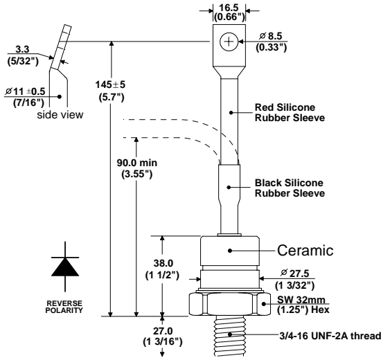
Base package conforms to JEDEC DO-9
